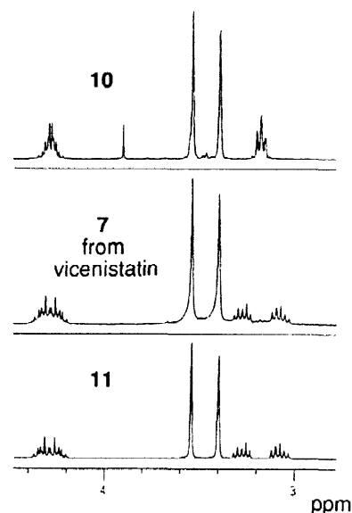
Fig. 4: ^1\text{H} -NMR Spectra of \text{C}_{15}\text{-C}_{19}
