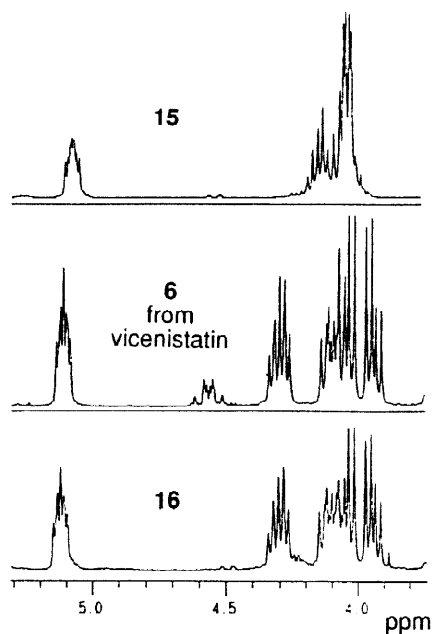
Fig. 6: ^1\text{H} -NMR Spectra of \text{C}_5\text{-C}_9
