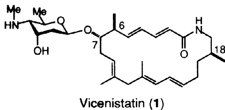
Fig. 7 : Absolute Stereochemistry of Vicenistatin
